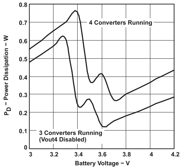
Figure 18. Power Dissipation vs Battery Voltage
